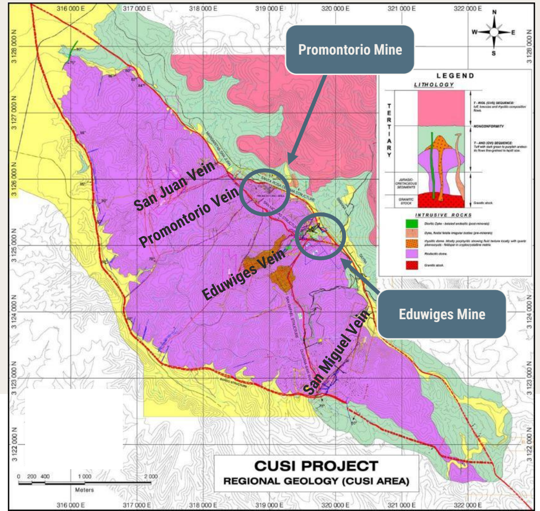
CUSI GEOLOGY AND VEIN MAP
